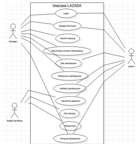
Gambar 8. Use Case Diagram
