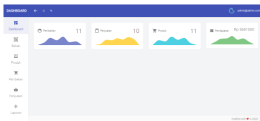
Gambar 12 Halaman Dashboard
