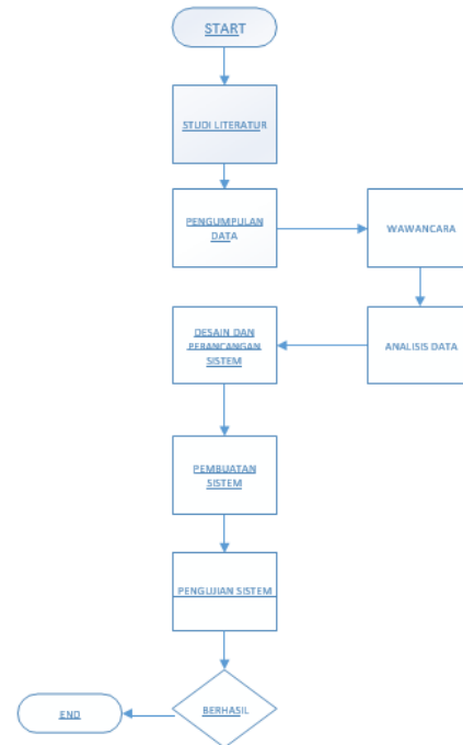
Gambar 2. Alur Penelitian
