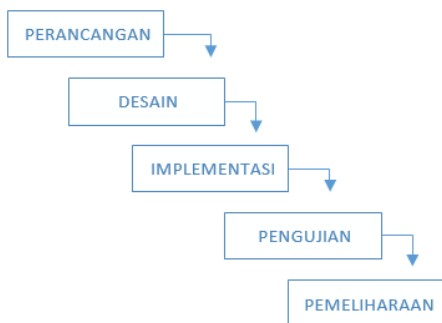
Gambar 1. Metode Waterfall
